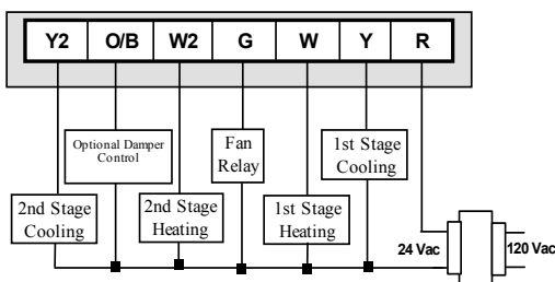
VIP 3000 Conventional System (Single Transformer)
