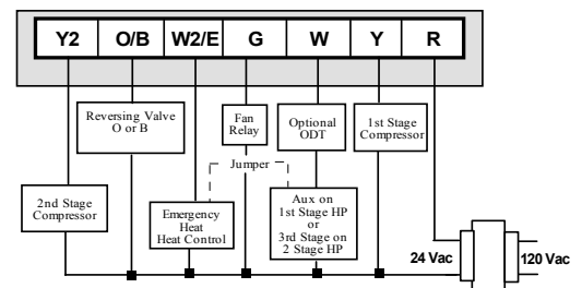
VIP 3000 Heat Pump Systems (Single Transformer)
